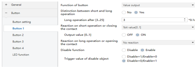
Figure 3.9"Button X- Value output "Parameter setting interface.
